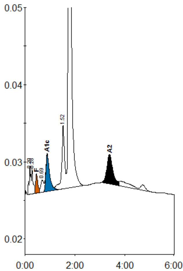
Peak table - ID: 11222465
