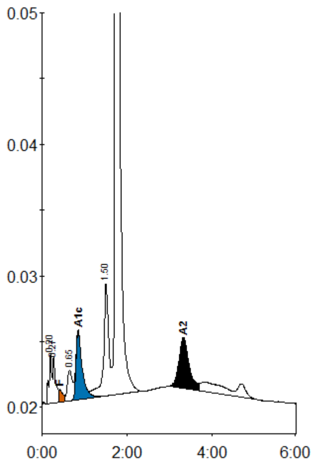
Peak table - ID: 11110945
